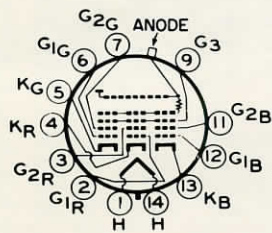
14AH ANODE = G_4 + G_5 + CL + R FOCUSING ELECTRODE = G_3
