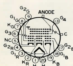
20A ANODE = G_5 + G_6 + CL FOCUSING ELECTRODE = G_3
