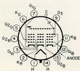
14BE ANODE = G_4 + G_5 + CL FOCUSING ELECTRODE = G_3
