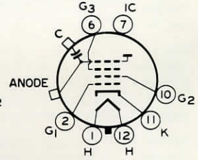
12C ANODE = G_4 + CL FOCUSING ELECTRODE = G_3
