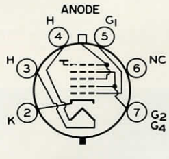
7FG ANODE = G_3 + G_5 + CL AUTOMATIC FOCUSING
