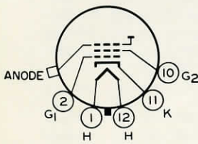
12D ANODE = G_3 + CL
