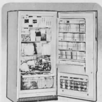
No. HU13-P* — G.E. "BOOK-SELF" FOOD FREEZER. Easy as taking books off a shelf. No rummaging, lifting with this convenient storage door. Puts twice as much food within finger-tip reach. Ice Cream Conditioner. Glide-out Basket designed for bulky, odd-shaped items. Juice Can Dispenser. Air-Vent Grille. 64" h, 30½" w, 26" d. LIST $419.95
