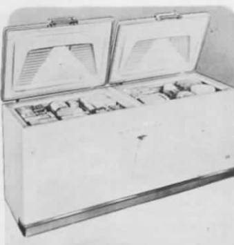
No. 7FK26 — HOTPOINT DELUXE CHEST-TYPE FREEZER. Holds 907 lbs. frozen food. Sliding baskets, vertical dividers, cake and pie rack. Twin Safety-type door. 36½" h, 84¼" w, 33" d. LIST $679.95. No. 7FK19. Same as above without twin door. 672 lbs. capacity. 36½" h, 60" w, 33" d. LIST $559.95.
