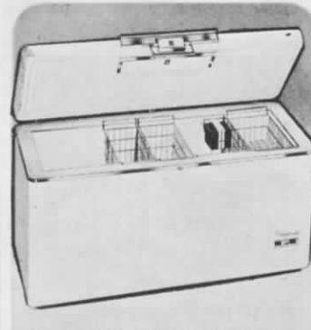
No. DI-20H* - RCA WHIRLPOOL IMPERIAL CHEST FREEZER. Captures the peak of flavor plus all other convenience and performance features. Automatic Temperature Control. Self-Aligning Counterbalanced lid. Spacious "on top" storage. 3 handy dispensers. Removable dividers. 37" h, 70 \frac{3}{8} " lg, 33 \frac{1}{8} " d. LIST $599.95.
