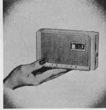
No. T-500 — PHILCO TRANSISTOR PORTABLE RADIO. Bantam, pocket-size 5 transistor set with 1 alloy junction audio and 4 surface barrier transistors. Built-in magnecor antenna. Private listening jack. Big-set sensitivity and output. 3¼" h. 6" w. 1½" d. Ivory. LIST $44.95.
