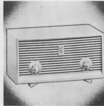
No. A508 — "PACEMAKER" TABLE RADIO — with built-in wavemagnet antenna, automatic volume control, front mounted control knobs, Zenith quality speaker. 5 1/4" h, 4 3/4" d, 9 3/4" w. Blue, Pink or Beige. LIST $21.95. Maroon. LIST $19.95.
