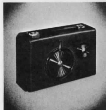
No. 676—PHILCO "SILVER SADDLE" PORTABLE RADIO. The sparkle of silver—the luxury of saddle leather. Engineered for long distance, sparkling tone reception on AC-DC or batteries. Unbreakable snap-open case, rugged as all outdoors. 6¾" h. 10" w. 4" d. Including batteries. LIST $53.10
