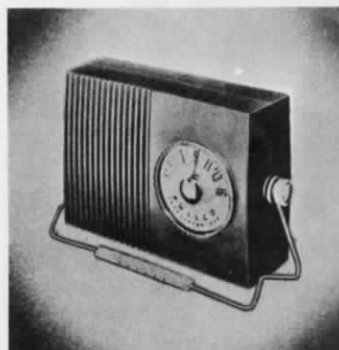
No. T-800 — PHILCO TRANSISTOR TABLE RADIO. Most versatile, multi-use 7 transistor set with 3 audio alloy junction and 4 surface barrier transistors. Oversize audio transformer. Unique stand and carrying handle locks in any position, or detached. 7¼" h. 10" w. 4" d. Turquoise. LIST $59.95.
