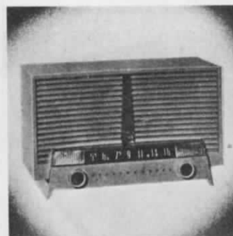
No. 435T5A - TABLE RADIO with sleek twin speaker, doubles your listening pleasure. Acoustically designed cabinet for room-filling sound. Push-Pull on-off switch - set and forget volume control. 5 tubes incl. Rectifier. 7" h, 11 1/4" w, 6 1/4" d. Available in Ivory, Tan or Green. $29.95
