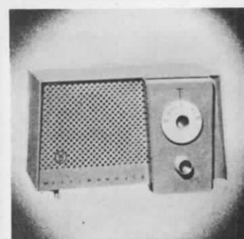
No. 629T4 - TABLE RADIO with famous Silver Safeguard Chassis. 4" Magna-Power speaker. 4 tubes incl. Rectifier. Tuning dial with large clear contrasting numerals for easy station selection. Big-set-like performer. 5 1/2" h, 9" w, 5 3/4" d. Ivory, Pink, Green. LIST $17.95
