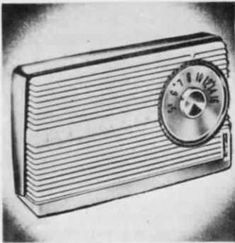
No. 8BT7* — RCA VICTOR "WINSOME" TRANSISTOR RADIO. A most happy choice — in size, sound and price. Its smart lines and beguiling color combinations make a really big impression anywhere. Two-tone Gray or in Turquoise and Antique White. 3¼" h, 5½" w, 1½" d. LIST $39.95.
