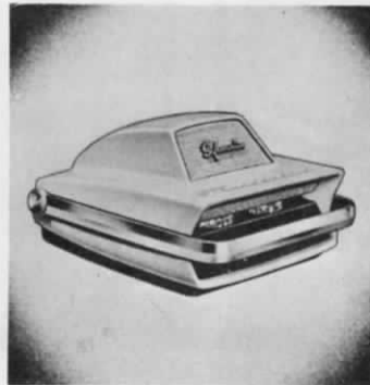
No. 3102 — SYLVANIA "THUNDER-BIRD" DELUXE 7 TRANSISTOR PORTABLE RADIO. Unique, years-ahead cabinet styling with sweeping modern lines. Unusual carrying handle designed into the unique styling. Lightweight 2½ lbs. 3¾" h, 5¼" w, 6¼" d. In two-tone Military Tan and Brown. Including batteries. LIST $75.00.
